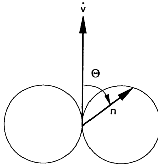
Figure 6.3. Angular distribution of radiation field of a nonrelativistic electron. The pattern is symmetric about the axis \hat{\mathbf{v}} .
