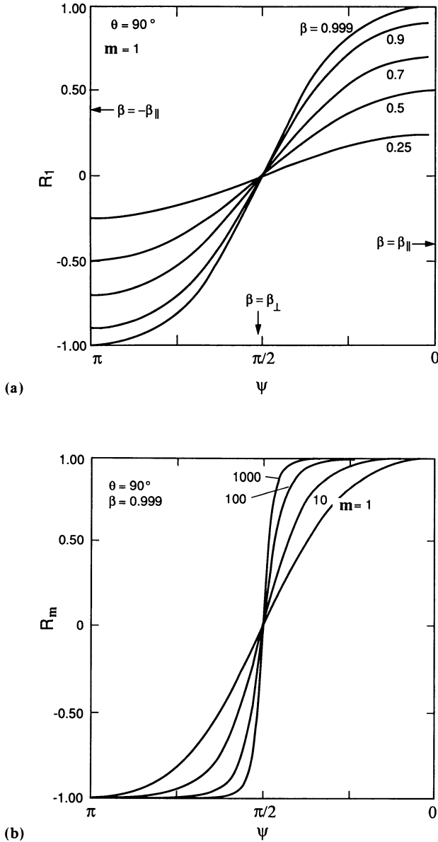
Figure 6.19. (a) R_l vs \psi for \theta = 90^\circ , \beta = 0.25, 0.5, 0.7, 0.9 , and 0.999 . (b) R_m vs \psi for \theta = 90^\circ , \beta = 0.999 , for m = 1, 10, 100 , and 1000 . (c) R_m vs \psi for \theta = 45^\circ , \beta = 0.999 , for m = 1, 10, 100 , and 1000 . (d) R_m vs \psi for \theta = 20^\circ , \beta = 0.999 , for m = 1, 10, 100 , and 1000 .
