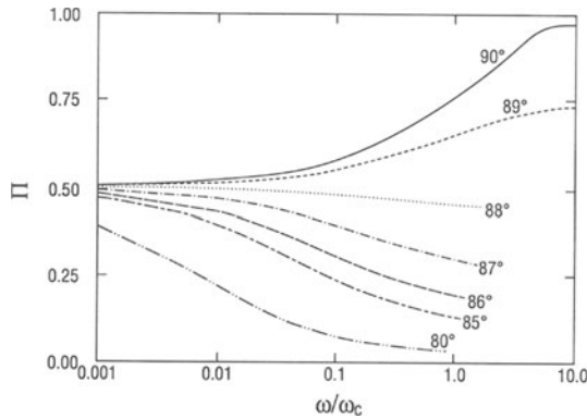
Figure 6.20. Polarization factor \Pi vs \omega/\omega_c .
