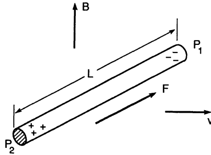
Figure 3.7. Induced voltage (potential drop between P_2 and P_1 ) in a conductor moving across a magnetic field.
