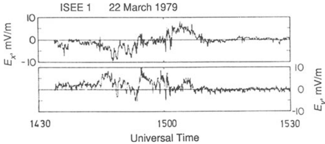
Figure 4.10. The field E measured in the plasmashet during a substorm active phase. (Courtesy of C.-G. Fälthammar).
