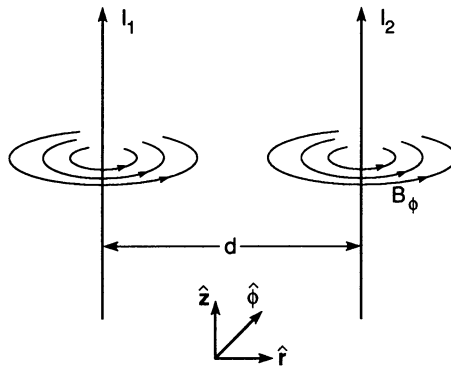
Figure 3.4. Two parallel current-carrying filaments.
