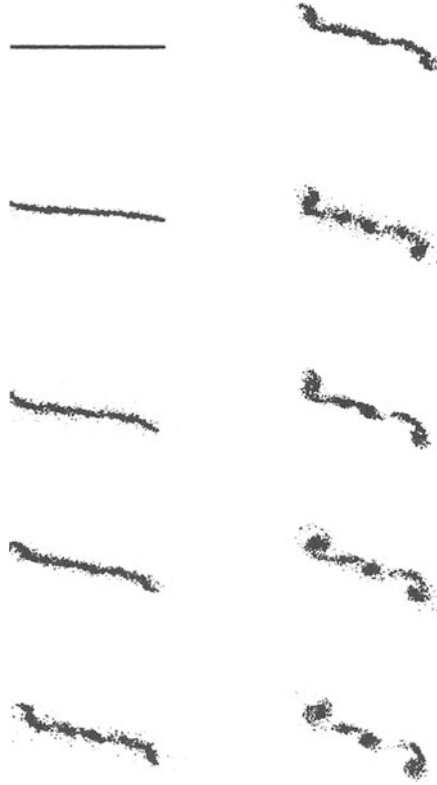
Figure 2.28. Simulated aurora. Current increases continuously from top to bottom in each column. The simulated beam is analogous to the experimental conditions leading to the data shown in Figure 2.15.
