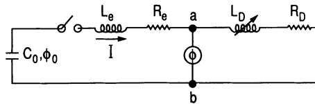
Figure 4.23. Equivalent electrical circuit of the plasma gun discharge. The subscripts e and D denote external and discharge circuit elements, respectively.
