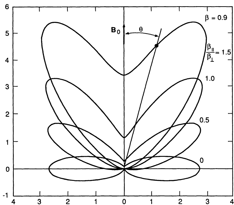
Figure 6.13. Gain patterns for \beta = 0.9 and \beta_{\parallel}/\beta_{\perp} = 0, 0.5, 1.0 , and 1.5 .
