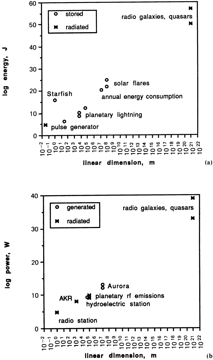
Figure 1.19. (a) Stored and radiated energies from man-made and natural plasmas versus linear dimension. Mankind's total energy consumption in 1989 is shown for comparison. (b) Generated and radiated power versus linear dimension.
