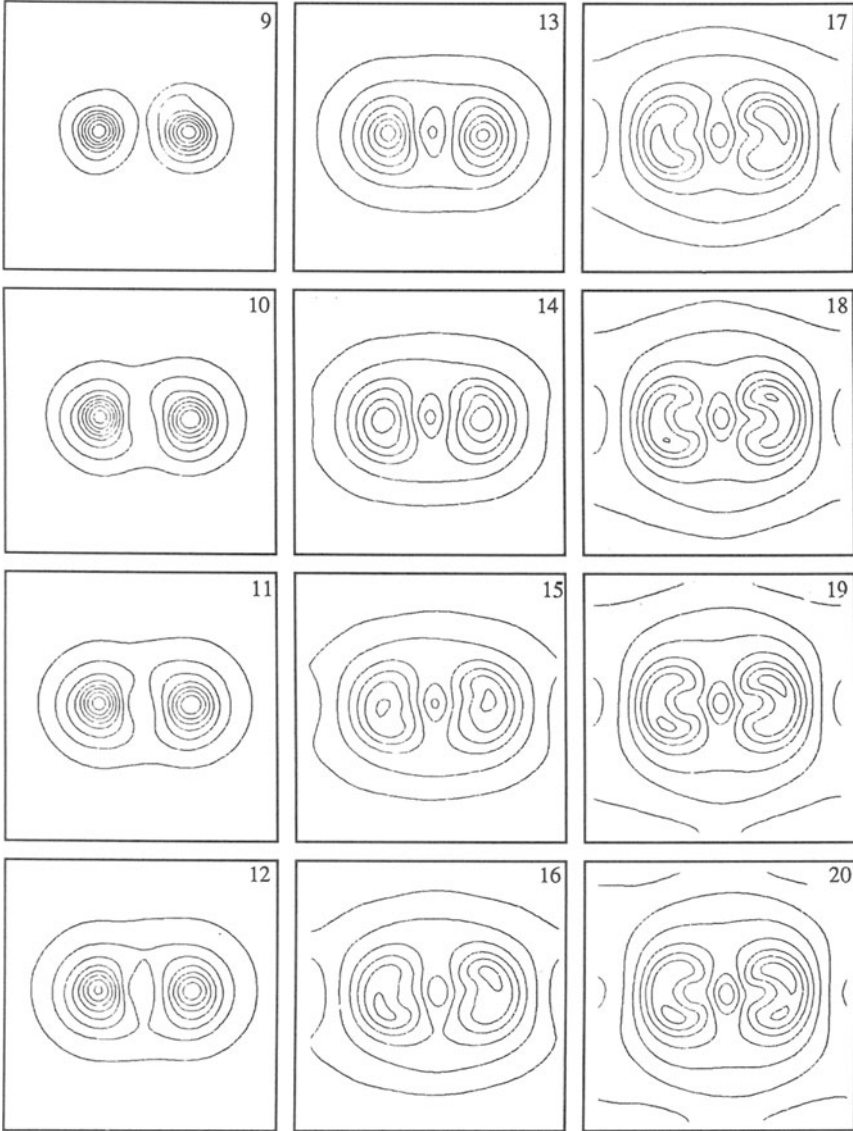
Figure 3.15. Contours of magnetic energy B^2 about two adjacent filaments at the simulation cross-section. T = 9-20 in 1 \Delta t steps. The contours at the locations of the two filaments correspond to energy maxima while the central ellipse is an energy minimum. “Hot spots” in azimuthal field energy feeding synchrotron radiation are beginning to become noticeable in later time frames.
