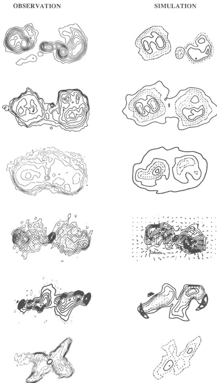
Figure 6.27. (right) Electric energy isophotes E^2 . Top to bottom: simulation times T = 51, 52, 236, 237, 280 , and 288 \, dt' , respectively. (left) Synchrotron isophotes (various frequencies) of double radio galaxies and quasars. Top to bottom: 0844+319, Fornax A, 3C310, 2355+490, 3C192, and 3C315.
