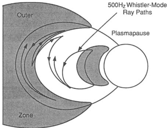
Figure 7.4. Example of 500 Hz whistler-mode ray paths, obtained from a ray tracing program, that illustrates how wave energy generated in the outer region of the plasmasphere can propagate across magnetic field lines so as to fill the plasmasphere with waves.
