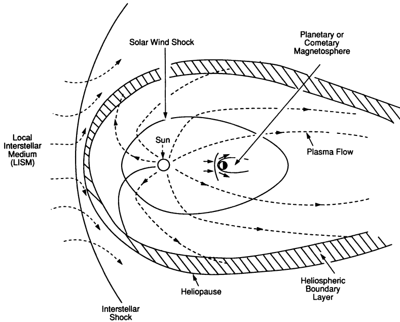
Figure 1.11. The heliosphere.
