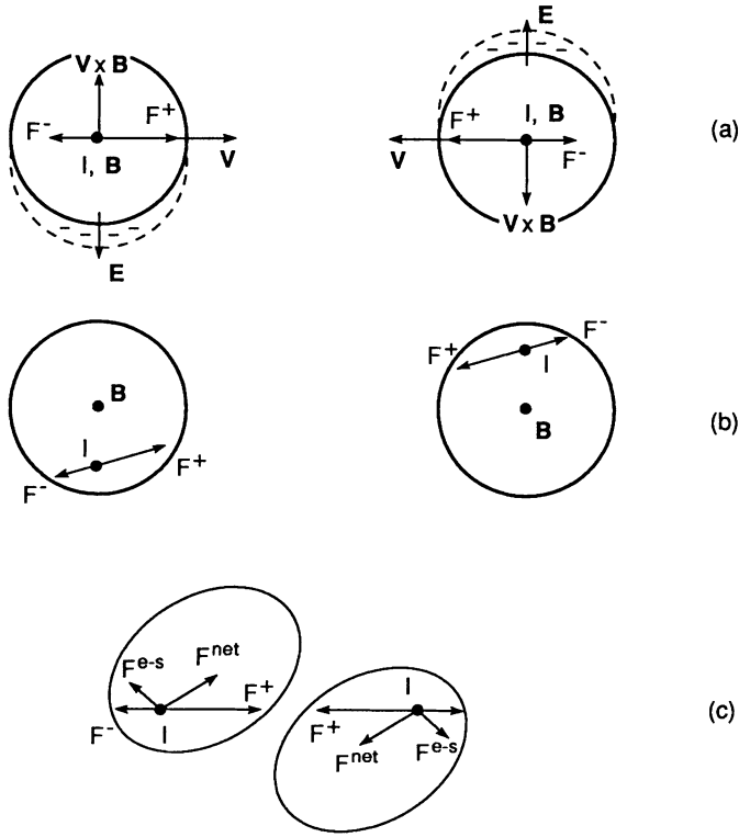
Figure 3.14. Net motion between adjacent Birkeland currents. (a) Polarization fields \mathbf{E} due to \mathbf{v} \times \mathbf{B} forces. (b) Net forces at early time (c) Net forces during filament distortion.
