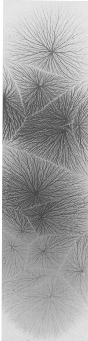
Figure 4.19. Lichtenstein figures recorded on the surface of an acrylic insulator used in a terawatt pulsed-power generator.
