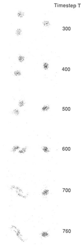
Figure 3.21. Interaction of three Birkeland filaments. Same parameters as Figure 3.19.
