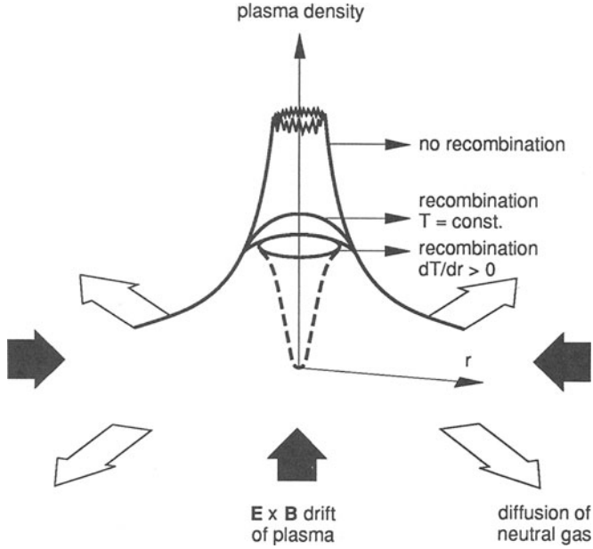
Figure 4.29. Plasma density profile as a function of radius sketched qualitatively for three cases: No recombination, recombination with T = \text{constant} , and recombination with a lower central temperature.
