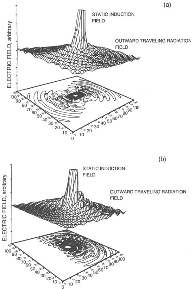
Figure 6.5. Induction and radiation fields E . (a) Single dipole radiator, (b) two dipoles spaced \delta = 1/8 \lambda apart. The dipoles are oriented in the plane along axes running from the upper left to the lower right.
