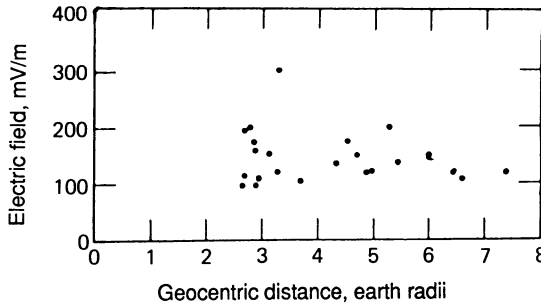
Figure 4.7. Peak electric field strengths in electrostatic shocks observed with ISEE-1. (Courtesy of C.-G. Fälthammar).
