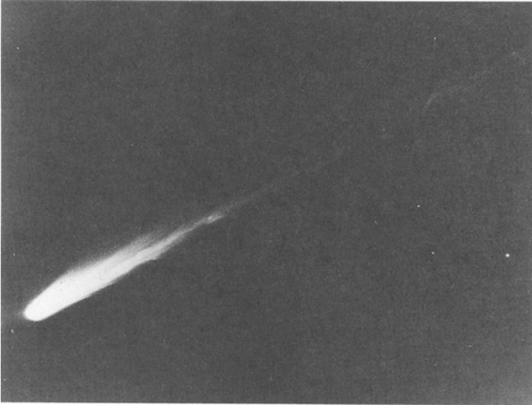
Figure 1.8. Comet Kohoutek (January 1974). The filamentary structure of the tail is typical of the structure of plasmas in space.
