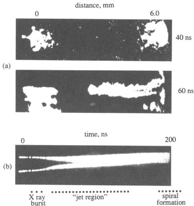
Figure 3.18. (a) Schlieren photographs of plasma light from of two interacting current-carrying plasma filaments (Z pinches) at times 40 and 60 ns, respectively (end view). The pinches are produced by exploding two parallel, 15 mm diameter, stainless steel wires with 250 kA of current. The two space frames show that plasma from the right-hand side filament has been channeled towards the central core, by the magnetic field isobars, at a velocity of about 100 km/s. The process is slightly asymmetrical: Plasma from the right-hand side filament has reached and filled the core at time 60 ns, whereas the plasma from the left-hand side filament has not yet started to move inward. (b) Streak camera photograph showing time evolution of interacting Z pinches conducting 667 kA (side view). A slit focused the midsections of the wires onto the film (cf, Figure 6.21). Three distinct regions are recorded: A radiation burst lasting about 5 ns, a “jet” region lasting about 50 ns, where plasma from the exploded wires is channeled inwards [as well as change in the circular cross sections (Figure 3.19)] and then, a spiral region, where the filaments rotate about each other. Reference is made to Figure 1.15 for a similar radiation pattern in astrophysical plasma.
