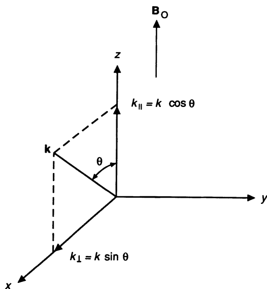
Figure B.2. The propagation vector \mathbf{k} in relation to the static magnetic field \mathbf{B}_0 .
