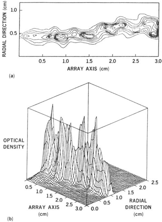
Figure 6.24. (a) Planar contour plot of a pinhole photograph from a titanium plasma. (b) Isometric plot of the optical density.
