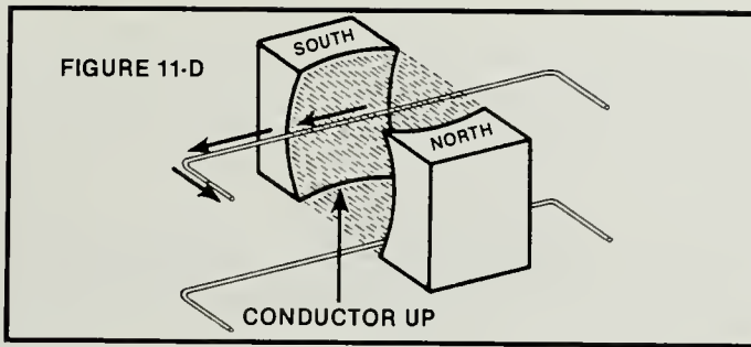
Figure 11-D Repeat the actions of Figure 11-B and the current flow will be left and opposite to Figure 11-B even though the force direction is the same.
